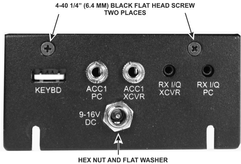
Figure 38. Mounting the Left Side Panel Part 2.
