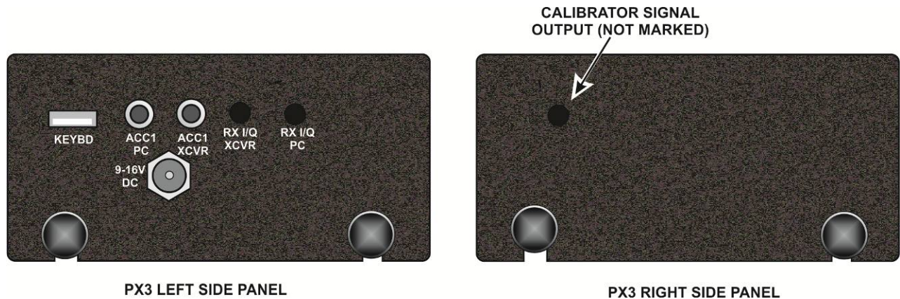
Figure 6. PX3 Side Panels.
